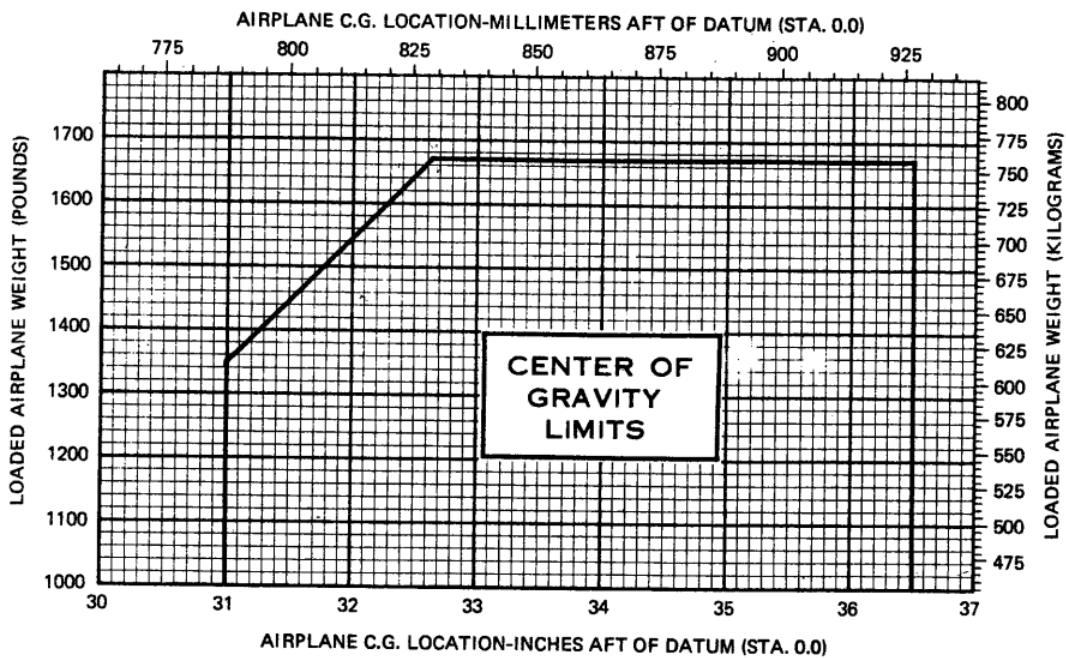
Figure 6-9. Center of Gravity Limits
