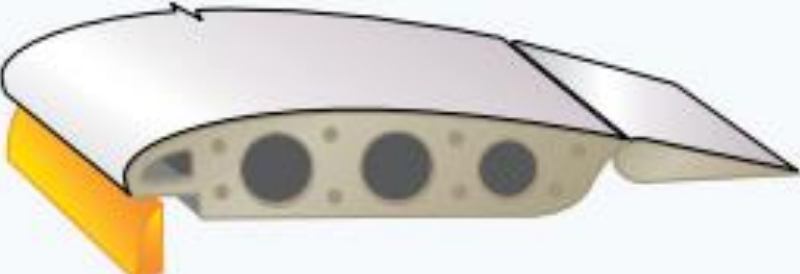
Leading edge flap
